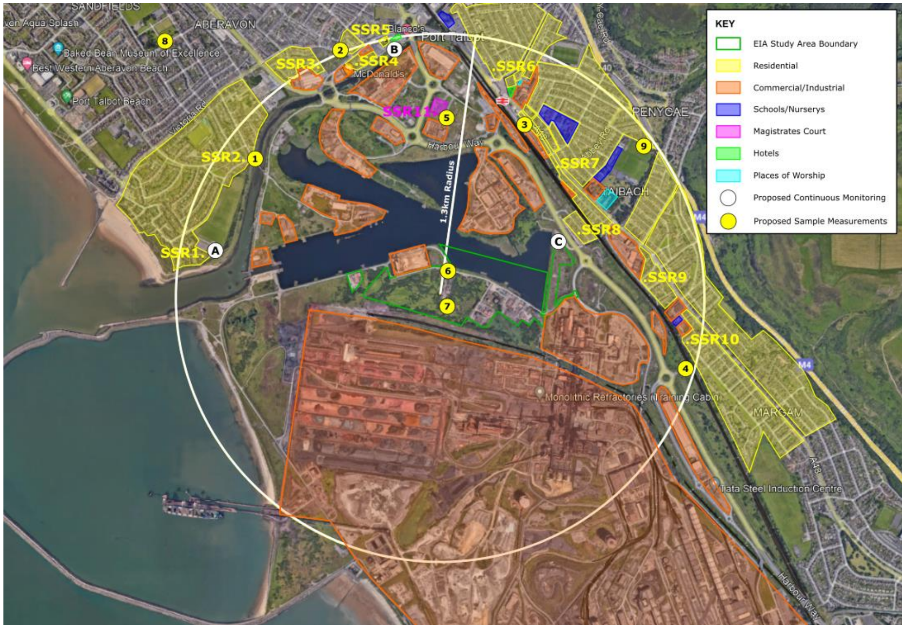
Figure 12.1: Noise Technical Study Area with Proposed Baseline Continuous Monitoring Locations
